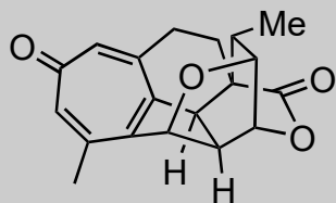
(+)-harringtonolide
