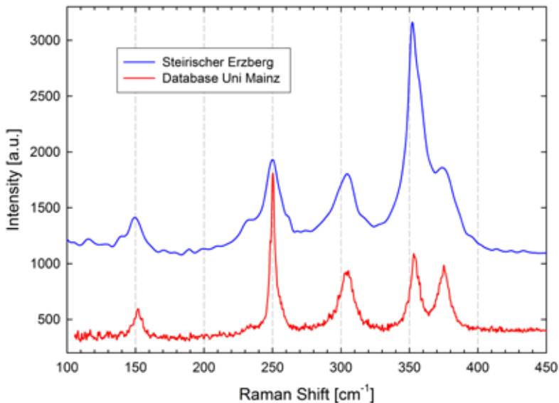
Figure 6. Raman spectra of millerite from the „Steirischer Erzberg“ and from the mineral Raman database of the University of Mainz, Germany (L. Nasdala, pers. comm.).
