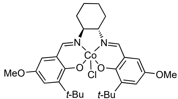
Co-salen complex
