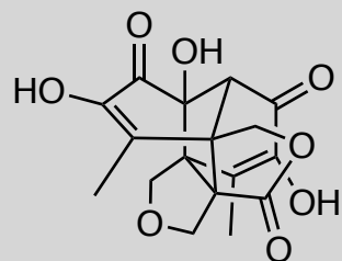
Epicolactone
