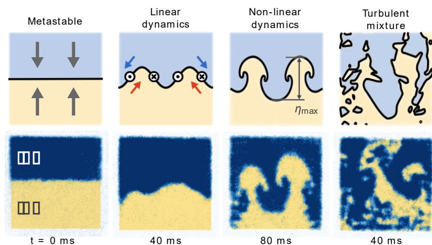
Evolution of the Rayleigh-Taylor instability. The upper panels present schematics, while the lower panels display corresponding experimental results. Component 1 is shown in yellow, and component 2 depicted in blue. Figure adapted from Geng et al.
