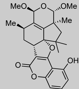
Hypocrolide A
