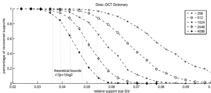
Figure 1: Comparison of Numerical Recovery Rates and Theoretical Recovery Bounds
