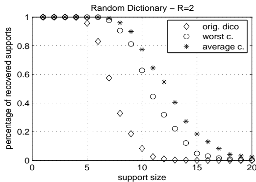
Figure 2: Recovery Rates for Different Sensing Dictionaries
