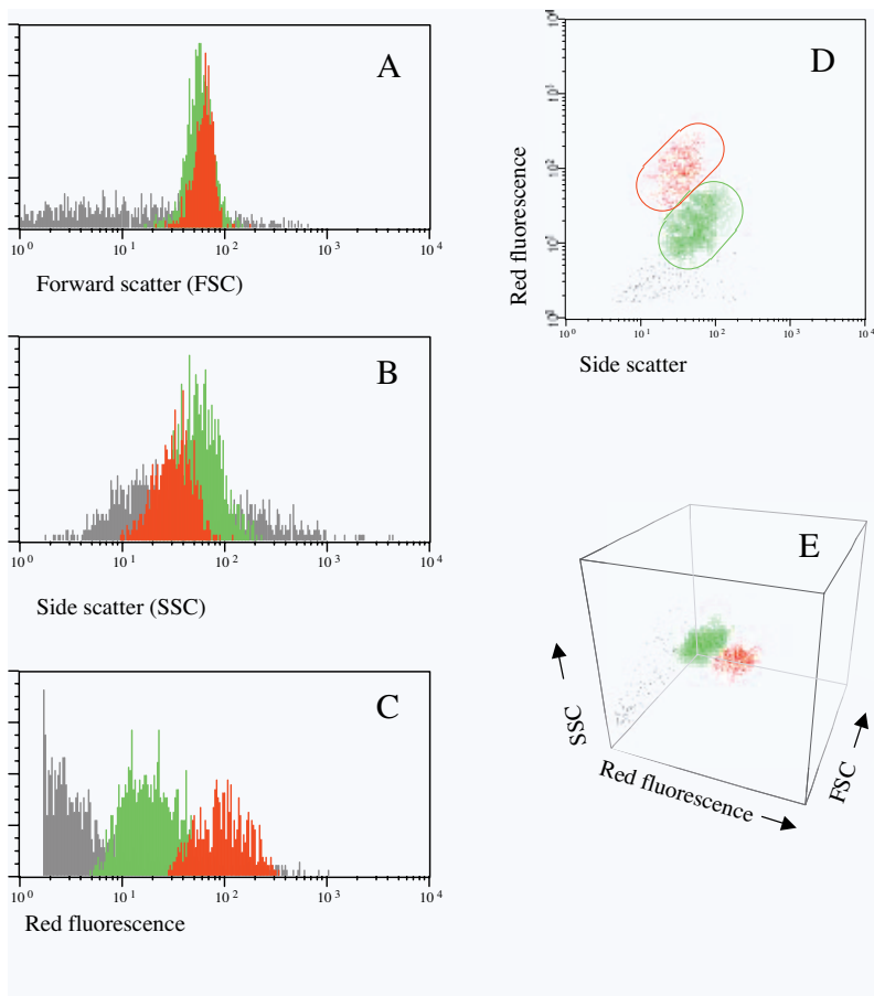
Fig. 2A-E: Flow cytometric analysis of individual cells of a natural sample taken from an acid mining lake (pH = 2.9) at Langau, Lower Austria, at 3 m depth on August 29, 2007. Forward scatter (FSC, A) is a measure of cell size, side scatter (SSC, B) is related to size and surface properties of the cells, red fluorescence indicates the cellular chlorophyll a content. All parameters were measured after logarithmic amplification in relative units. The red population represents the green alga Chlamydomonas acidophila , the green population the mixotrophic chrysoomonad Ochromonas sp. The histograms show that both populations largely overlap in their cell size (A, B) and also, to some extent, in their autofluorescence (C). The populations can be discriminated unequivocally in the red fluorescence vs. side scatter dot plot (D) and in the three-dimensional plot (E). Each dot in D and E denotes one individual cell. The flow cytometer used was a FACS Calibur (Becton Dickinson) equipped with an Argon laser.
