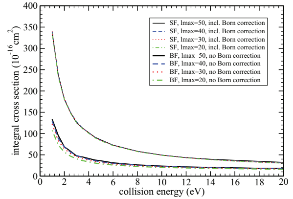
FIG. 7. (Color online) Computed integral cross sections for positron scattering off gas-phase pyrimidine using different partial wave expansions. The thick lines in the lower part represent computations in the body-fixed (BF) frame. The thin lines are the calculations done in the space-fixed (SF) frame including Born dipole correction and summation over rotational elastic and inelastic channels.
