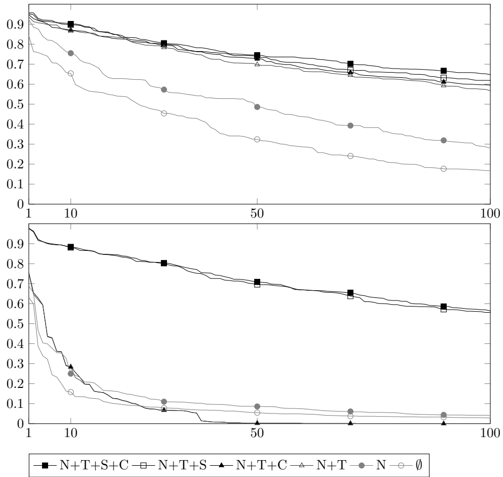
Figure 4: Effect of normalization when aligning Coq with Mizar (top figure) and HOL Light with Isabelle/HOL (bottom figure). “N” stands for CNF normalization + logical AC. “T” stands for default typing formation. “S” stands for subterm conceptualization. “C” stands for the fourth level of AC normalization which includes permutation of arguments in non-commutative constants.
