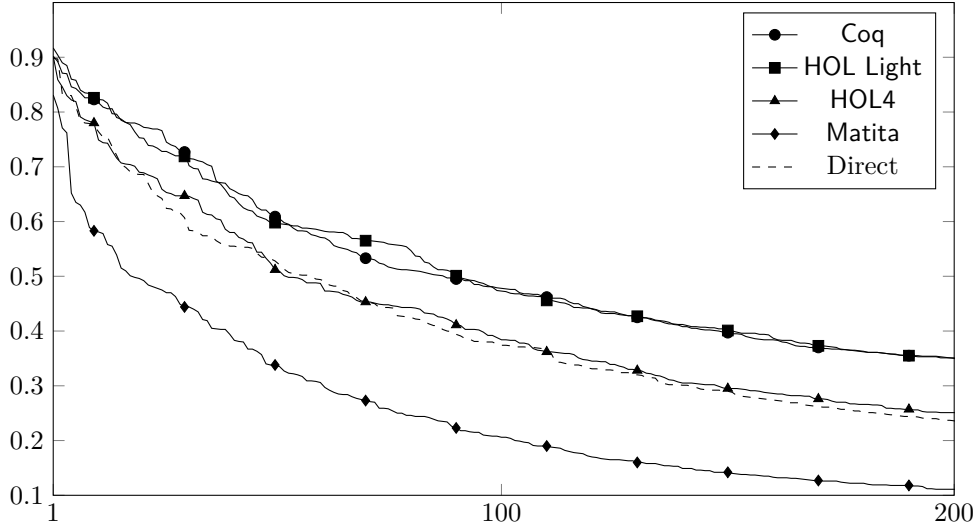
Figure 6: Best transitive matches between Isabelle/HOL and Mizar.
