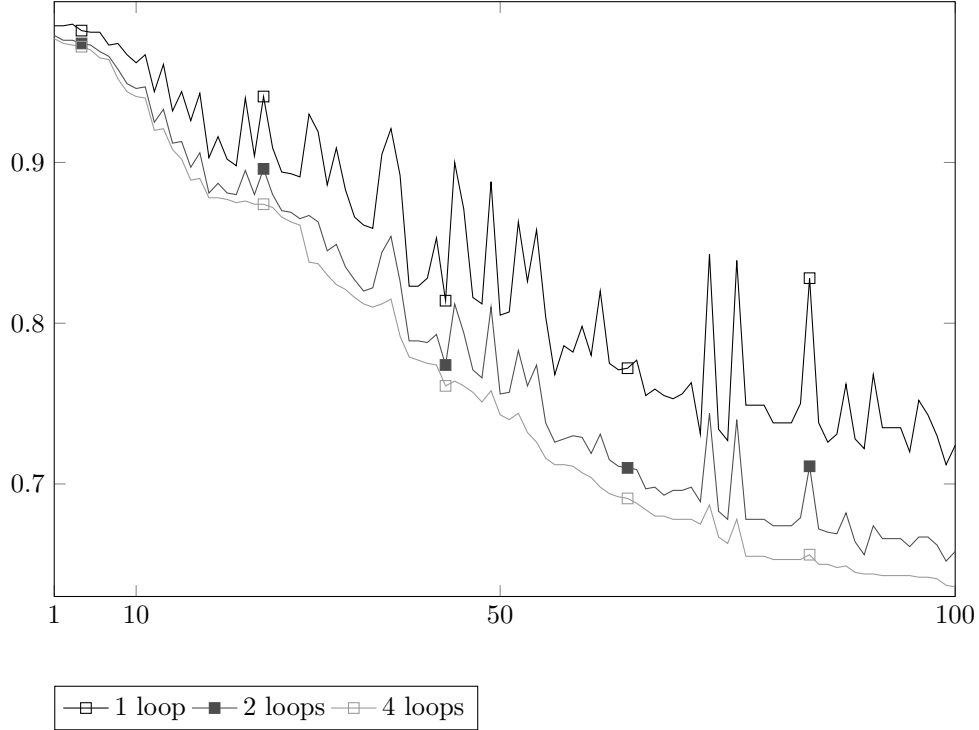
Figure 3: Scores of the best 100 constant pairs when matching Coq with HOL4 after 1,2,4 loops, ordered by their rank after 16 loops. The graph after 16 iterations is not presented here as it would be very close to the 4 loops curve.
