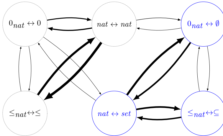
Figure 2: Part of the correlation graph of Isabelle/HOL-Mizar matches with stronger correlations drawn with wider arrows.
