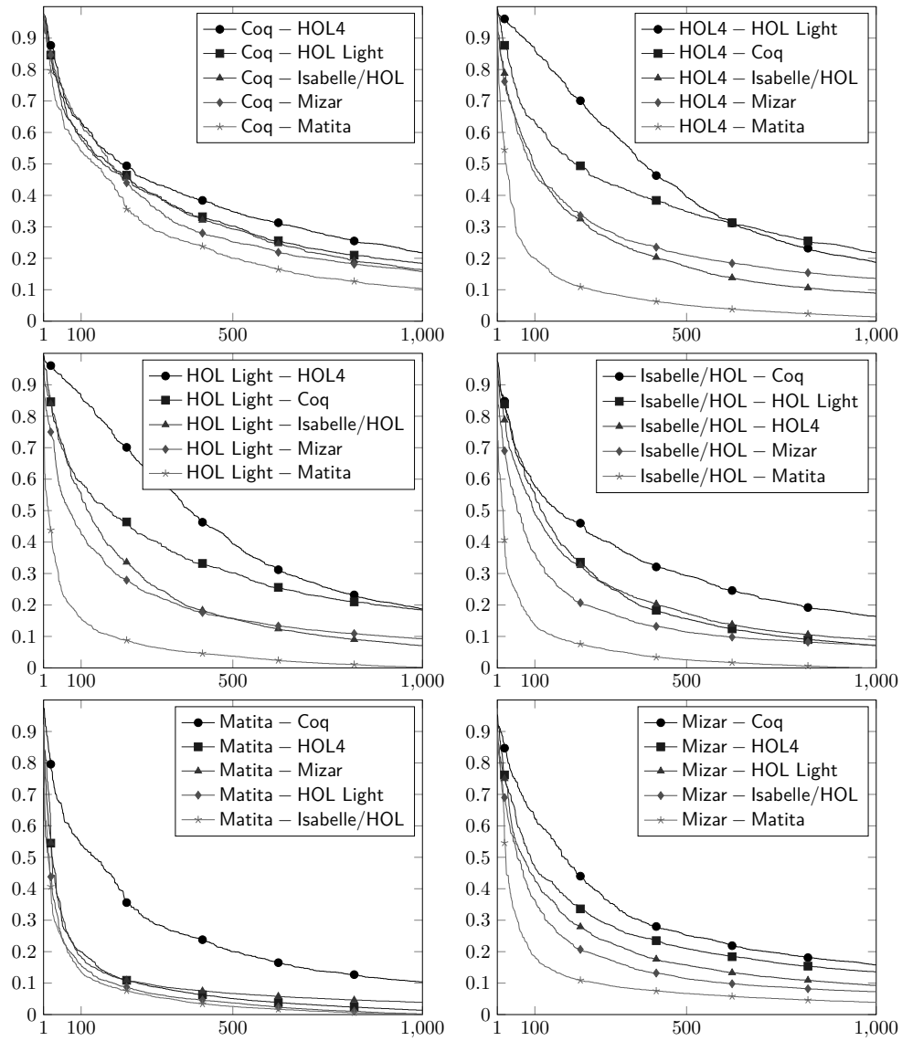
Figure 5: Scores of the best thousand pairs of constants with default settings.
