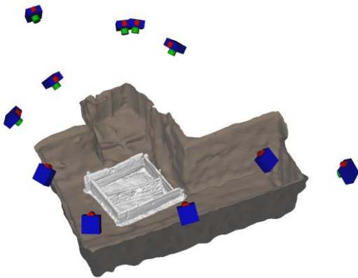
Figure 3: The last stage of excavation, positions of the digital cameras after their relative and absolute orientation
