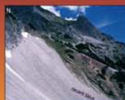
Fig. 3. The talus breccia at Tasseid (background) is linked to the actual geomorphic setting of the recent talus deposits (foreground).
