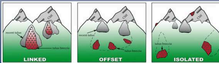
Fig. 1. Schematic illustration of the geomorphic relation of talus relicts to their present day setting.
