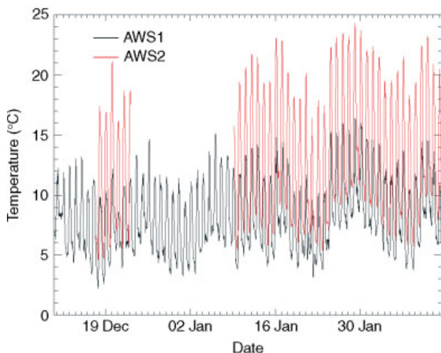
Figure 3. Comparison of hourly measurements of air temperature (°C) at the two automatic weather stations on (AWS1) and close to the glacier (AWS2). AWS2 started recording later than AWS1 and did not work in the period 23 December 2005–9 January 2006, see Table I
