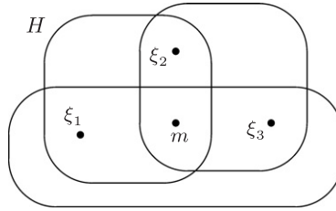
Fig. 6. The median property.
