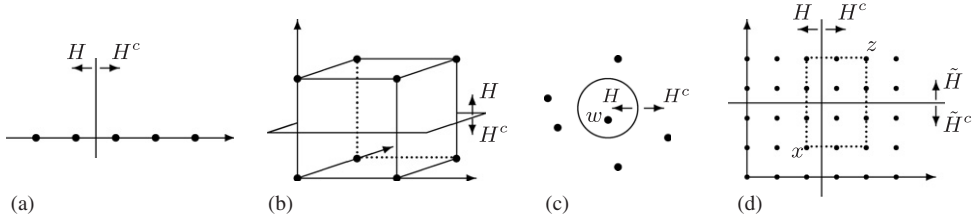
Fig. 2. Basic properties underlying Examples 1–4.
