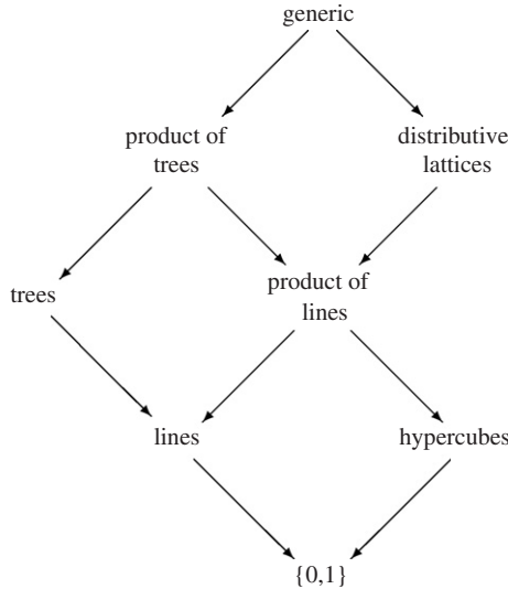
Fig. 8. The class of median spaces.
