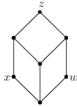
Fig. 7. A seven point graph.
