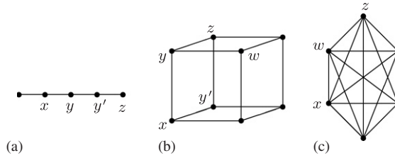
Fig. 1. Three graphic betweenness relations.
