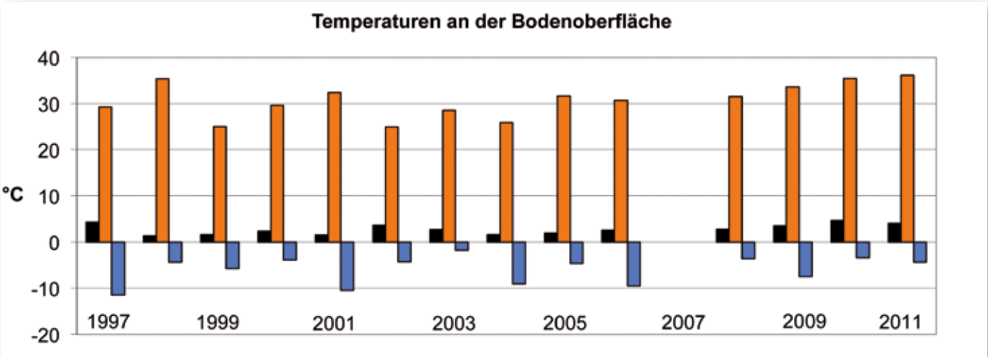
Temperatures on the surface of the 1971 moraine: annual mean (black), absolute maxima (orange) and minima (blue) in the period 1997-2011. Data are missing for 2007 since data loggers failed.
