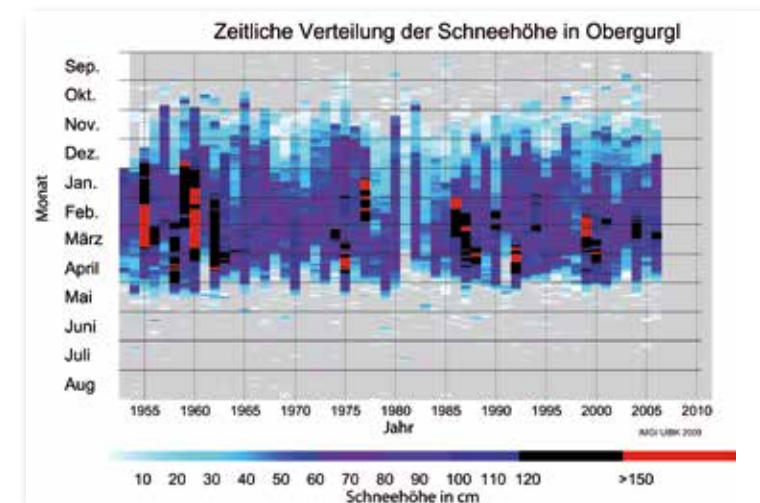
Depth of the snow in Obergurgl from 1953 to 2006
