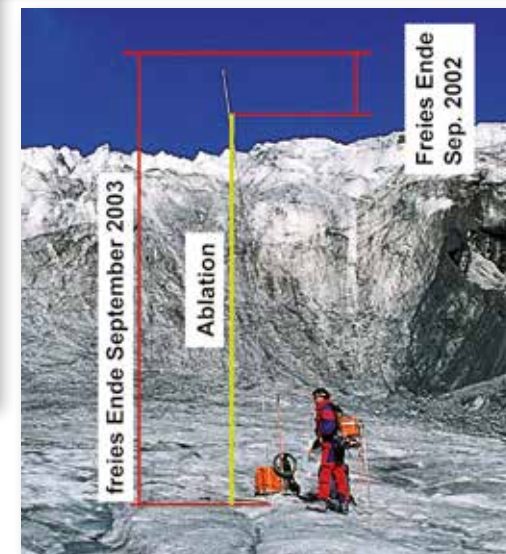
Glaciological mass balance programs comprise measurements of ablation at gauges and accumulation at snow shafts (photo: A. Fischer)
