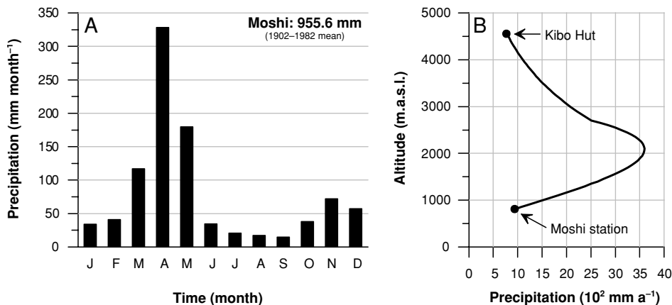
FIGURE 12.1. (A) Mean annual cycle of precipitation at Moshi (813 m a.s.l.), equatorial East Africa, 1902–82, and (B) vertical distribution of annual precipitation on the southern slope of Kilimanjaro. Data from the Global Historical Climatology Network climate data set (Vose et al. 1992); vertical distribution derived from the precipitation-altitude relation after Røhr and Killingtveit (2003), with Moshi as reference station.
