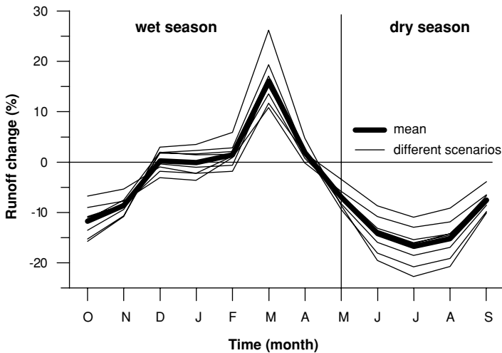
FIGURE 12.8. Changes in future runoff in the Llanganuco catchment area, Peru, with respect to runoff for 1961–90 (after Juen, Georges, and Kaser 2005). Thin lines represent calculations based on different climate scenarios for either 2050 or 2080 (see Juen, Georges, and Kaser 2005 for details), while the bold line shows the cycle of change averaged over all scenarios. The time axis follows the hydrological year (i.e., starts with October).
