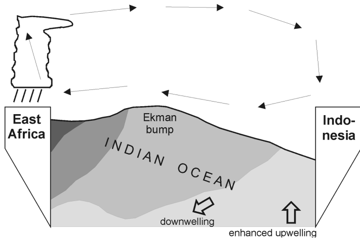
FIGURE 12.6. Vertical cross section at latitude 5°S illustrating ocean-atmosphere mechanisms of the anomalously strong East African short rains of 1997 (after Webster et al. 1999). The color scale from light to dark gray denotes increasing sea temperature; arrows indicate the direction of the atmospheric circulation.
