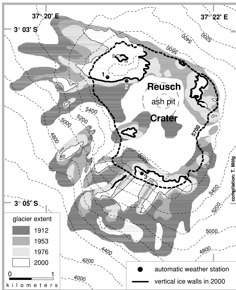
FIGURE 12.3. Glacier extents on Kibo in 1912, 1953, 1976, and 2000 (Hastenrath and Greischar 1997; Thompson et al. 2002); map contours in meters, UTM zone 37 projection. Also shown are the locations of the automatic weather stations (1–3) and the distribution of vertical ice walls (Mölg, Hardy, and Kaser 2003). The highlighted 5,700-m contour delimits Kibo’s summit plateau approximately. Dashed circles indicate the conical Reusch Crater. Map compiled by T. Mölg, January 2003/December 2004.
