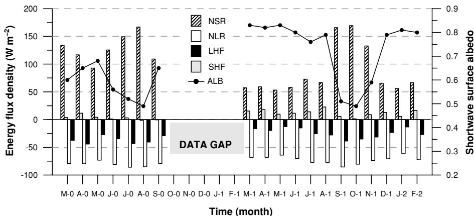
FIGURE 12.5. Energy-balance components at the weather station on the Northern Icefield between March 2000 and February 2002. NSR , Net shortwave (solar) radiation; NLR , net longwave radiation; LHF , turbulent latent heat flux; SHF , turbulent sensible heat flux; and ALB , shortwave albedo of the glacier surface. Positive values indicate energy gain for the surface, negative ones energy loss. For details of calculation see Mölg and Hardy (2004).
