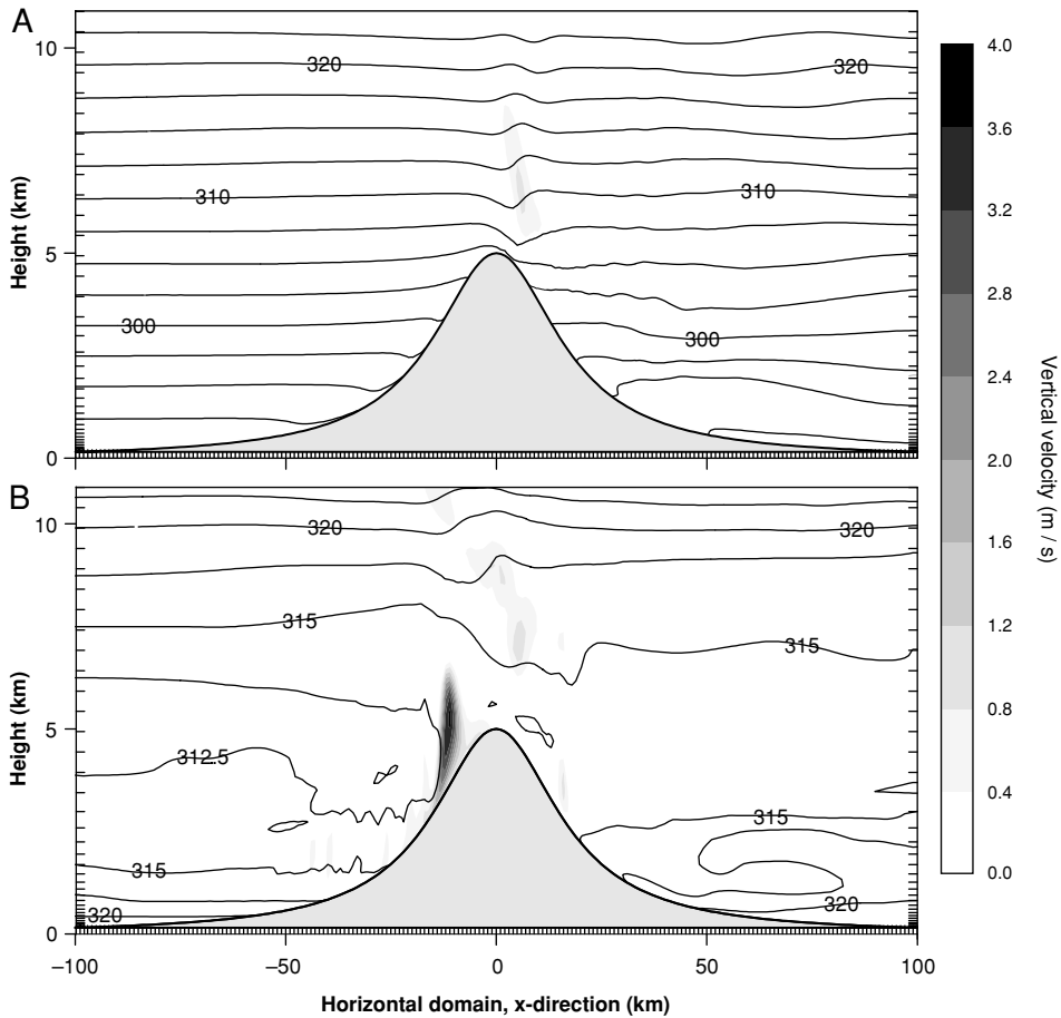
FIGURE 12.7. Vertical cross section of air flow past an idealized Kilimanjaro massif after six hours of integration in a 3-D model atmosphere: (A) dry with 0% relative humidity (RH), and (B) wet (RH = 100% until 5,000 m a.s.l., then linear decrease to 0% at 10,000 m a.s.l.). Shown are isolines of equivalent potential temperature (isentropes) with a 2.5-K spacing and gray-shaded contour surfaces of the upward-directed component of vertical velocity (spacing 0.4 m/s). Air flow follows the isentropes approximately and is from left to right with a constant background flow of 10 m/s. Note the vertical exaggeration of the plots.
